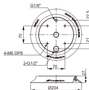
LF200-12F
